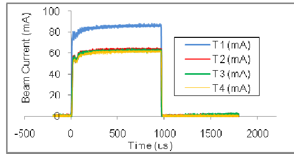
FIG 8: 62 mA beam current profiles at 50 Hz 1 ms. (1.2 ms 60 A discharge, 19.6 kV extraction voltage, 65 keV beam, 180°C caesium oven, 16 mLmin -1 H 2 )
