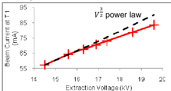
FIG 3: Beam current vs extraction voltage.
