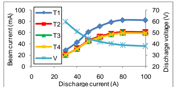
FIG 5: H^- beam currents and discharge voltage vs discharge current.
