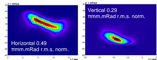
FIG 10: Beam emittance at the entrance of the RFQ for the beam shown in fig 8.
