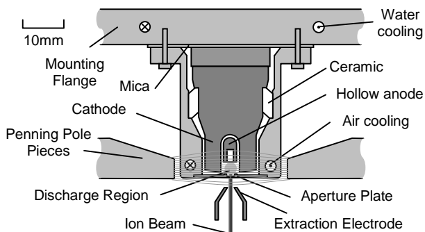
FIG 1: A schematic of the FETS ion source.
