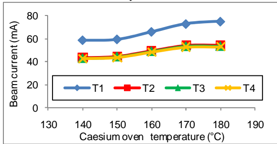
FIG 7: H^- beam currents vs caesium oven temperature for a 55 A discharge.
