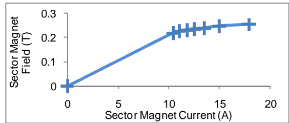
FIG 4: Sector magnet field vs current.
