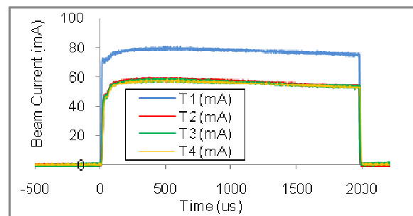
FIG 9: 60 mA beam current profiles at 25 Hz. (2.2 ms, 64 A discharge, 19.6 kV extraction voltage, 65 keV beam, 190°C caesium oven, 16 mLmin -1 H 2 )
