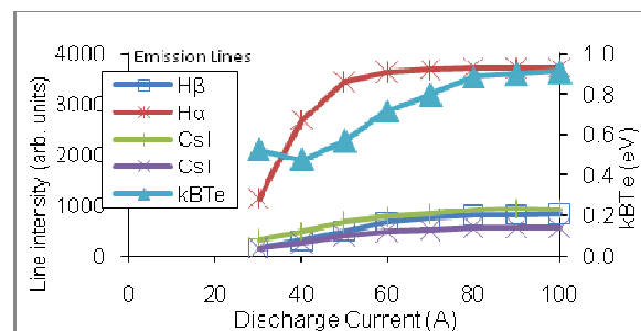
FIG 6: Optical emission peaks vs pulsed discharge current.
