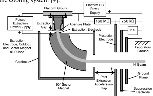
Figure 1: Schematic of the FETS ion source extraction and post acceleration system.
