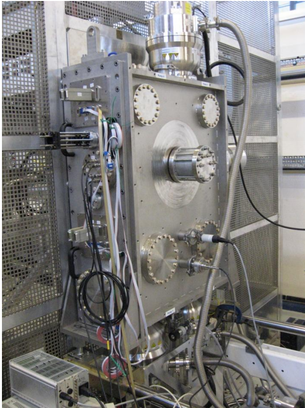
Figure 7: The ion source and laser diagnostics vessel.
