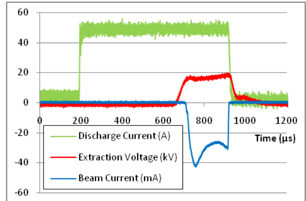
Figure 8: Oscilloscope traces showing the first beam produced by the front end test stand.
