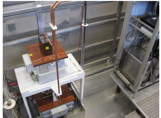
Figure 6: The single and three phase isolation transformers.
