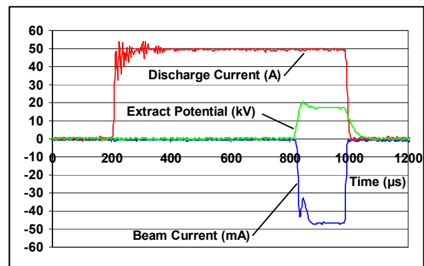
Figure 5: Scope traces for 4A Penning coil current.
