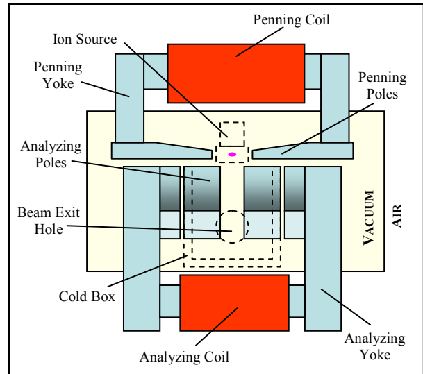
Figure 1: Schematic of the analyzing and Penning magnetic circuits.
