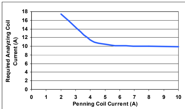
Figure 3: The analyzing coil current required for different Penning coil currents (17kV extract potential).
