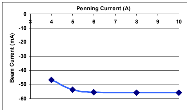
Figure 7: Variation of output beam current with Penning current.
