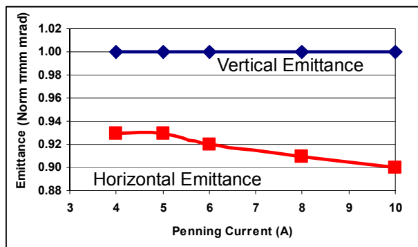
Figure 8: Variation of beam emittance with Penning coil current.
