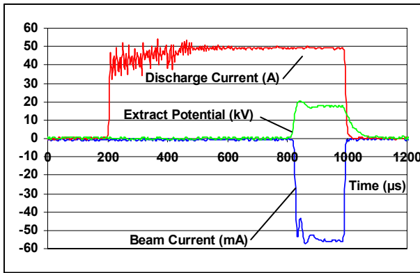
Figure 6: Scope traces for 10A Penning coil current.
