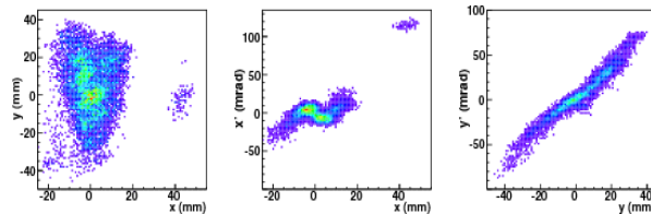
Figure 5: Spatial and phase space distributions in the transversal plane used as input for the LEBT transport simulations ( \epsilon_{x,rms}=0.81\pi\text{mmmrad} ; \epsilon_{y,rms}=0.97\pi\text{mmmrad} ) gained from measurements with the pepper pot device.
