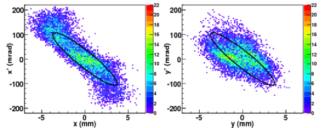
Figure 8: Phase space distributions in the transversal plane at the exit of the LEBT using the input data shown in Figure 5 ( \epsilon_{x,rms}=1.21\pi\text{mmmrad} ; \epsilon_{y,rms}=0.93\pi\text{mmmrad} ).
