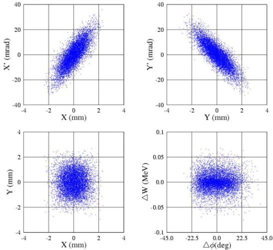
Figure 10: Particle distribution behind the RFQ for the input distribution shown in Figure 7 ( \epsilon_{x,rms}=0.35 \pi mmmmrad; \epsilon_{y,rms}=0.35 \pi mmmmrad, \epsilon_{z,rms}=0.19 \pi deg MeV).
