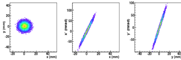
Figure 4: Spatial and phase space distributions in the transversal plane used as input for the LEBT transport simulations ( \epsilon_{x,rms}=0.25\pi\text{mmmrad} ; \epsilon_{y,rms}=0.25\pi\text{mmmrad} ).
