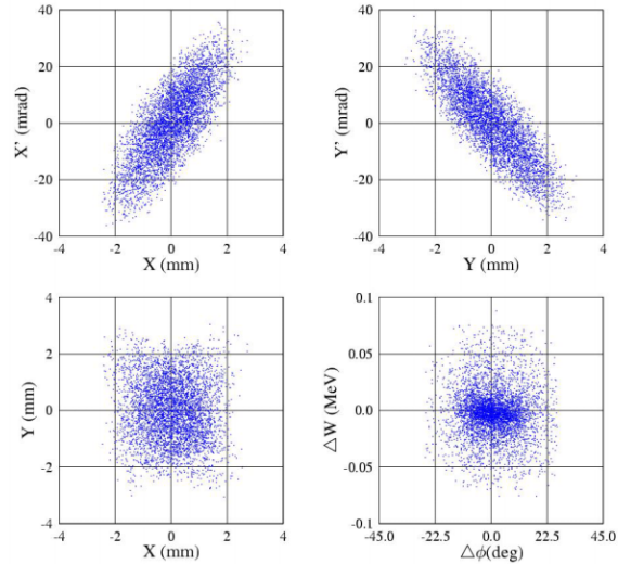
Figure 11: Particle distribution behind the RFQ using the input distribution shown in Figure 8 ( \epsilon_{x,rms}=0.62 \pi mmmmrad; \epsilon_{y,rms}=0.62 \pi mmmmrad, \epsilon_{z,rms}=0.21 \pi deg MeV).
