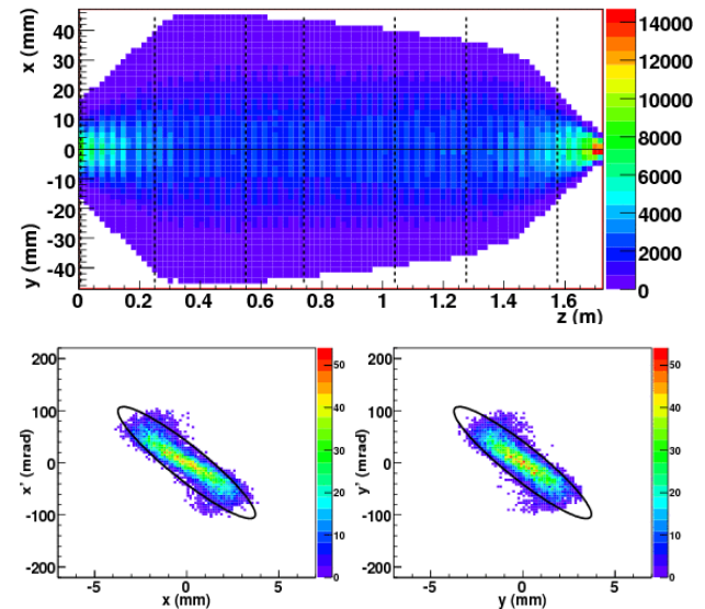
Figure 7: Trajectory plot (above) and output emittances in the transversal plane (below) based on LEBT simulations, using the input data shown in Figure 4 ( \epsilon_{x,rms}=0.33\pi\text{mmmrad} ; \epsilon_{y,rms}=0.33\pi\text{mmmrad} ).
