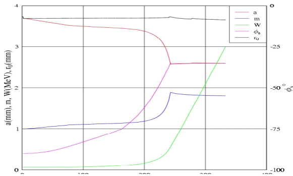
Figure 9: Development of the main RFQ parameters for the FETS along z.
